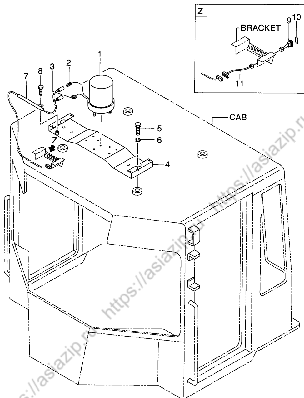
FIG. 22 REVOLVING LAMP (RLY001-648) (OP) 回転灯
