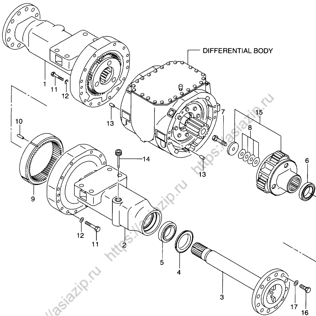
DRIVE AXLE - FRONT (1/3)
