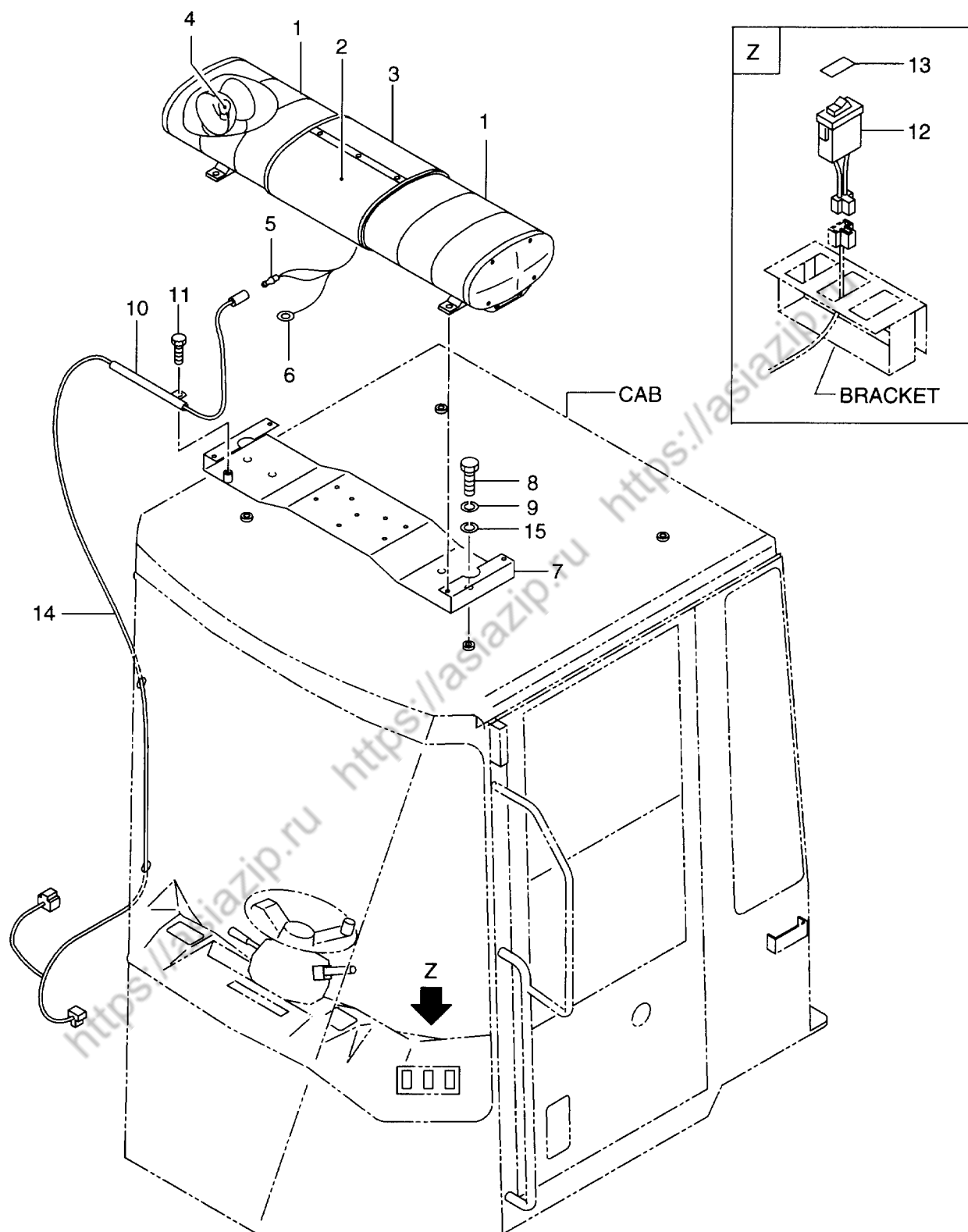
FIG. 25 REVOLVING LAMP (RLYS02-648) (OP) 回轉灯
